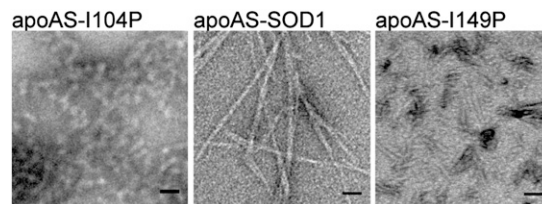
Fig. 5. Pro substitutions in ^{101}\text{DSVLSL}^{107} and ^{147}\text{GVIGIAQ}^{153} inhibited aggregation of full-length protein. Wild-type like apoSOD1 with mutated surface C6A and C111S (apoAS-SOD1) in which Ile104 was substituted with Pro, formed amorphous aggregates (Left). There were also occasional fibers like those of the wild-type protein (Center). Short rods were observed in the apoAS-SOD1 I149P sample (Right) together with some wild-type-looking fibrils.
