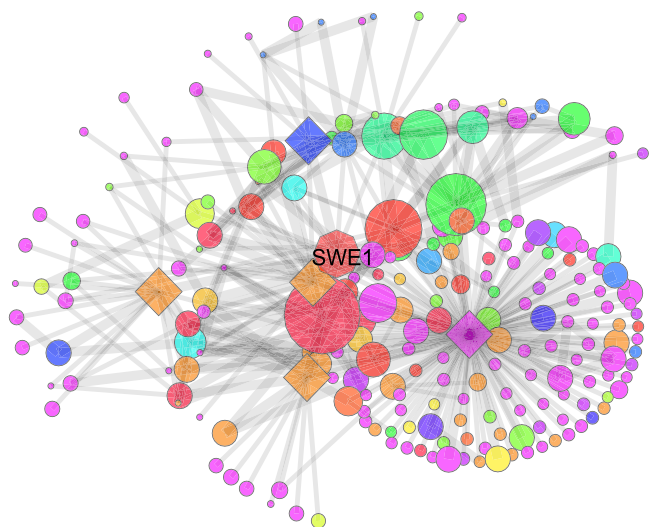
Fig. 2. Zorch quantifies connectivity to the target. An initial unit of zorch flowed from the target SWE1 throughout the protein-protein interaction network. Protein interactions identified by reliable small-scale experiments in DIP core (wide edges) allowed more flow than those from high-throughput experiments (narrow edges). Highly connected proteins accumulated more zorch (large nodes). Proteins shown to interact with SWE1 with edges in DIP core were removed to rigorously evaluate GFL annotation (diamonds). Despite the influence of many linked proteins with different functions (blue transport, green cytoskeleton organization, purple other), GFL combined prior information, the MF kinase activity of SWE1, with zorch-linked proteins involved in the cell cycle (red and orange), to successfully predict a correct biological process: regulation of cyclin-dependent protein kinase activity. Voting failed for SWE1.
